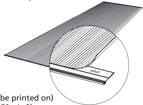
Art nr.: 4.55.08530-01, 4.55.10030-01, 4.55.12030-01, 4.55.15030-01 Material: nylon
